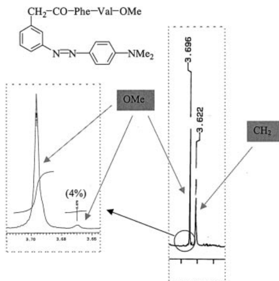
Figure 1. ^1\text{H} NMR spectrum of Ddp-Phe-Val-OMe ( 14c ) before purification
